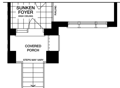
Partial Main Level ELEVATION C
