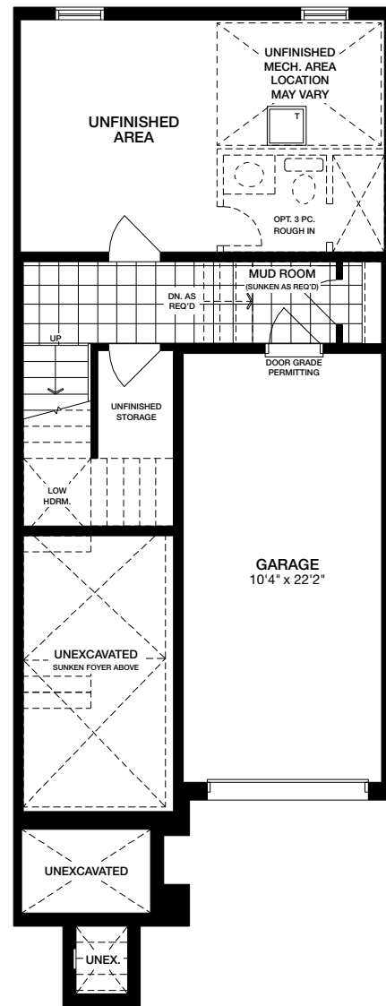
Ground Level ELEVATION A & C
