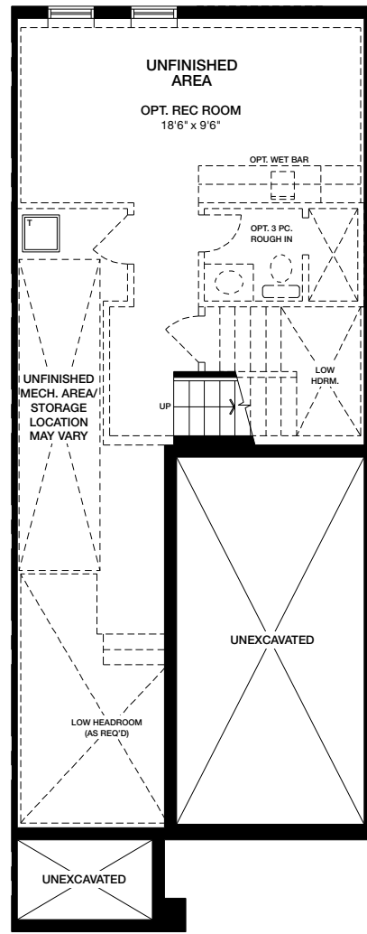
Lower Level ELEVATION A
