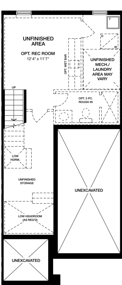
Lower Level ELEVATION A
