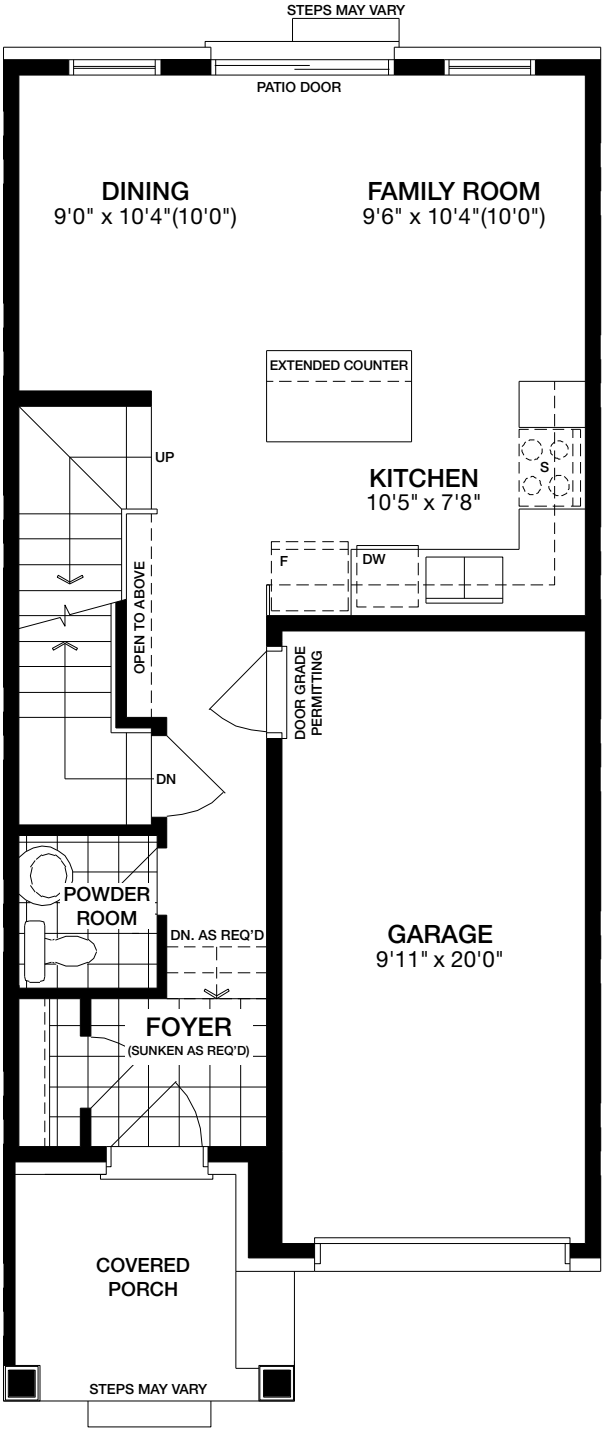
Main Level ELEVATION A
