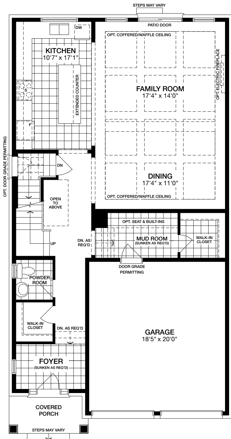
Main Level ELEVATION A
