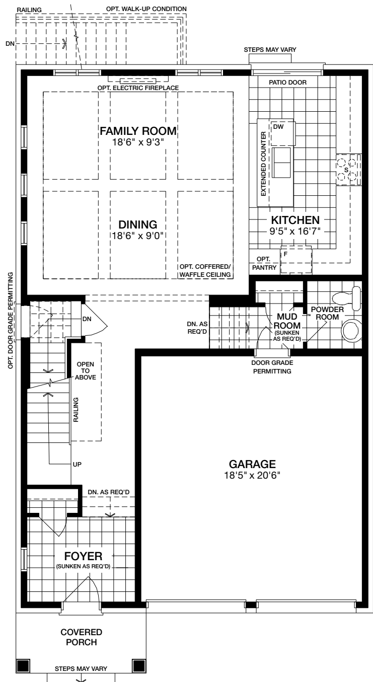
Main Level ELEVATION A
