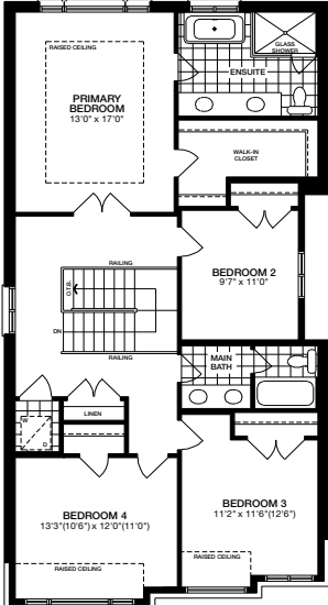
Opt. Upper Level With 4 Bedrooms ELEVATION C
