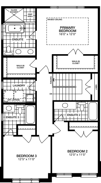
Upper Level ELEVATION B
