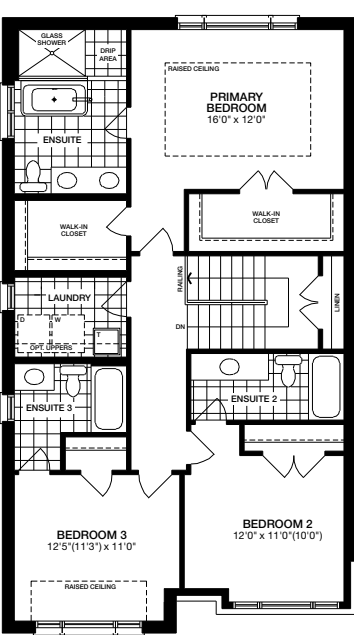
Upper Level ELEVATION C
