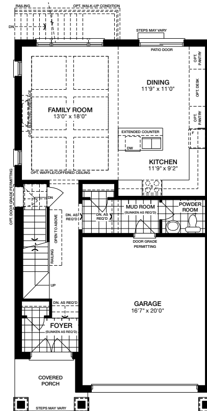
Main Level ELEVATION B
