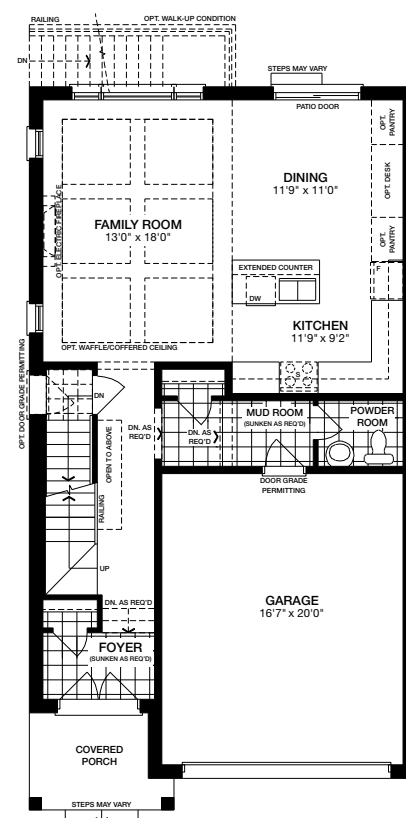
Main Level ELEVATION C
