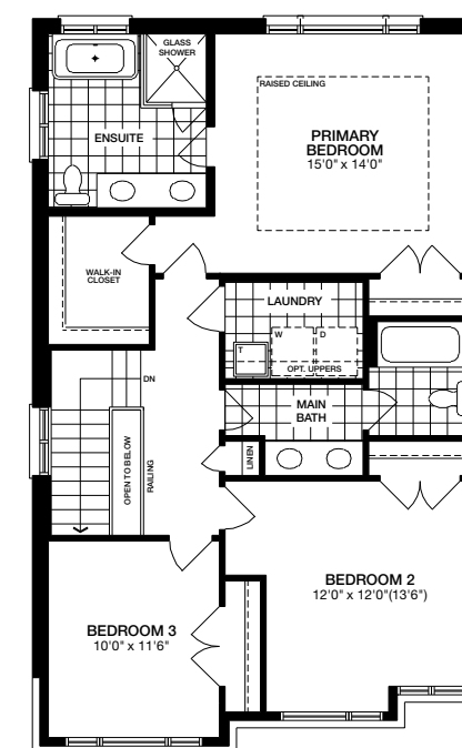
Upper Level ELEVATION C
