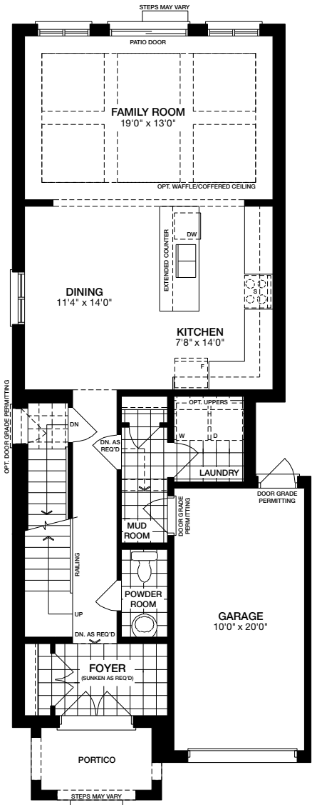
Main Level ELEVATION C
