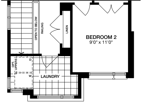
Partial Upper Level ELEVATION C
