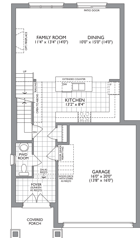
MAIN LEVEL ELEV. B
