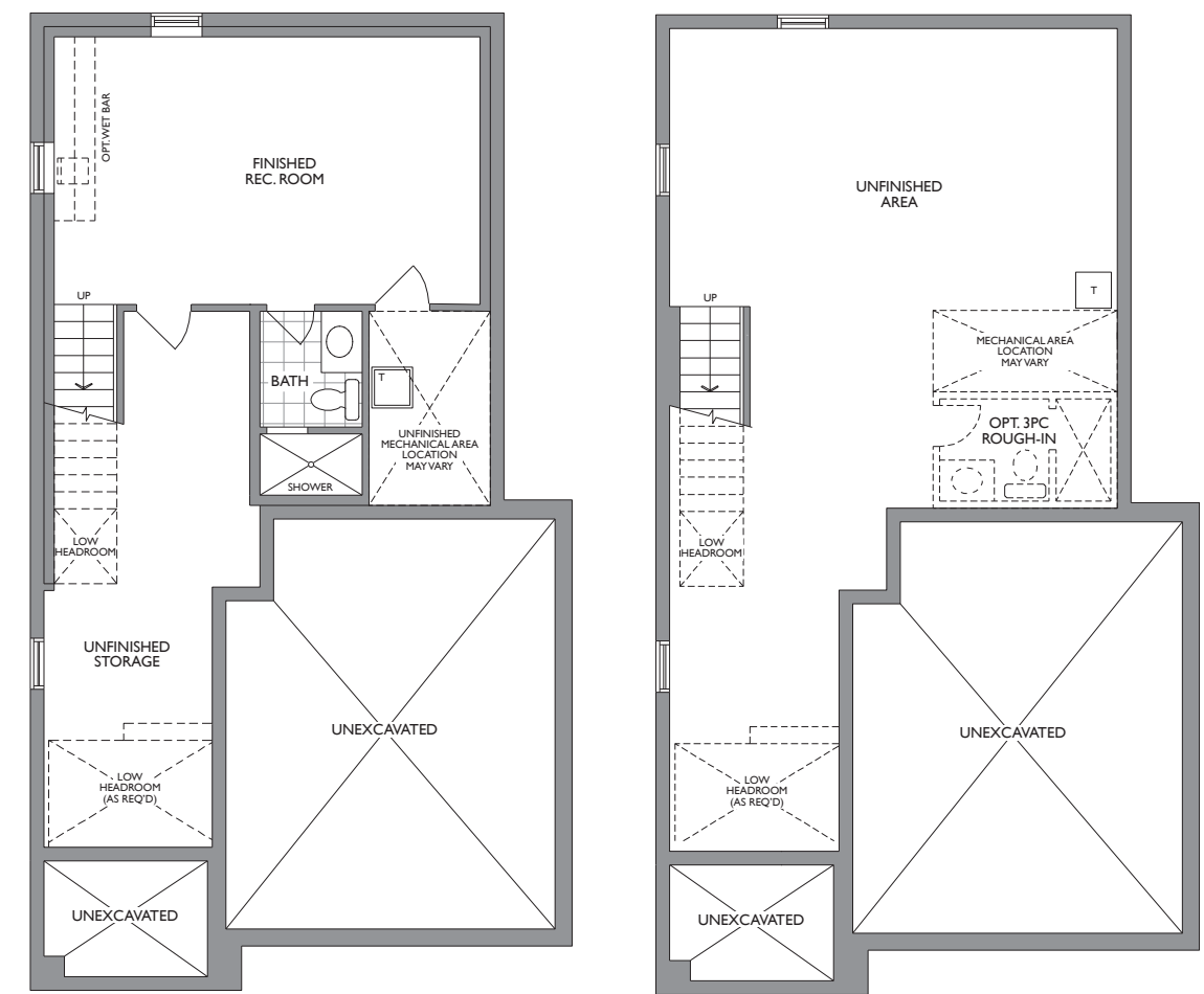
OPT. LOWER LEVEL WITH FINISHED REC. ROOM ELEV. A, B & C
