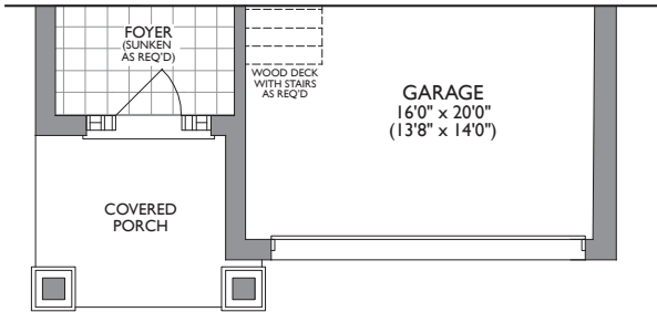
PARTIAL MAIN LEVEL ELEV. C
