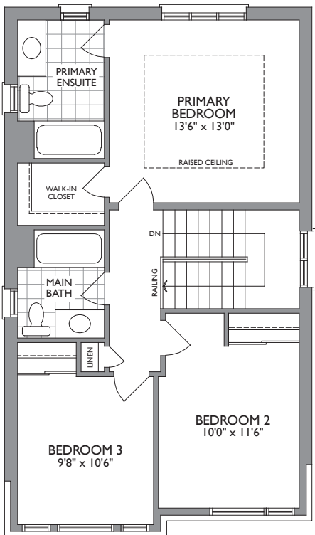
UPPER LEVEL ELEV. B
