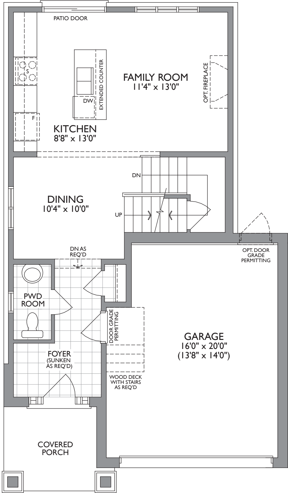
MAIN LEVEL ELEV. A
