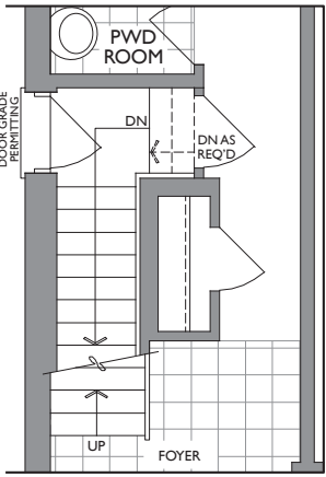
PARTIAL MAIN LEVEL WITH OPT. SIDE DOOR ELEV. A, B & C
