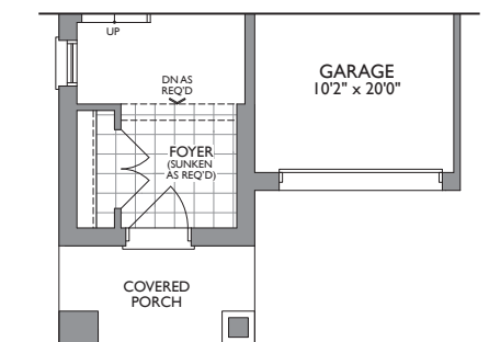
PARTIAL MAIN LEVEL ELEV. B
