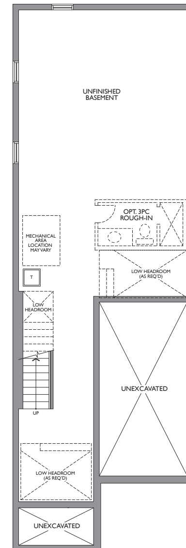
LOWER LEVEL ELEV. A
