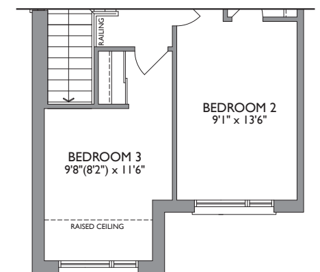
PARTIAL UPPER LEVEL ELEV. B
