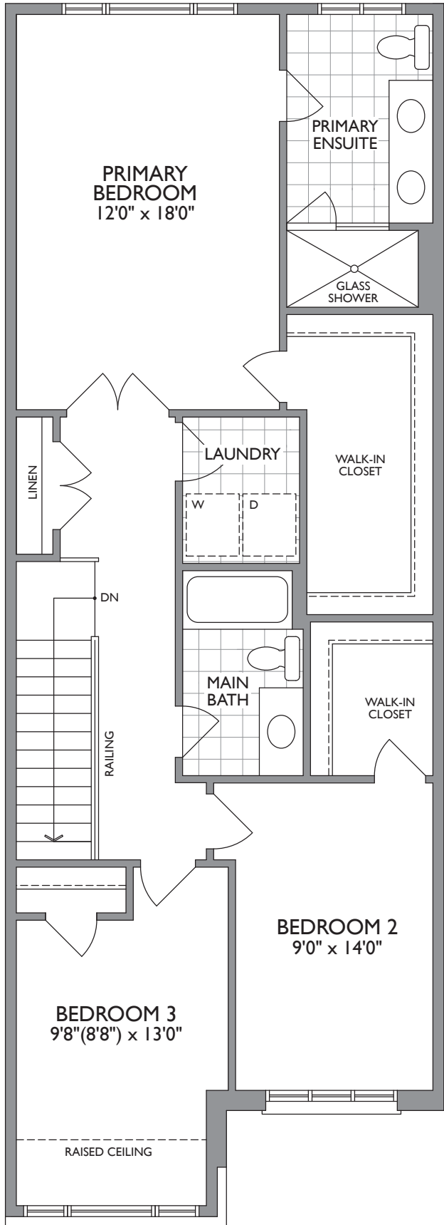
UPPER LEVEL ELEV. A
