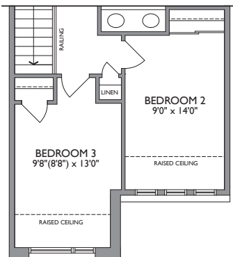
PARTIAL UPPER LEVEL OPT. 4 BEDROOM ELEV. B
