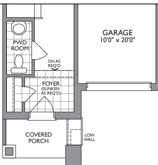
PARTIAL MAIN LEVEL ELEV. B
