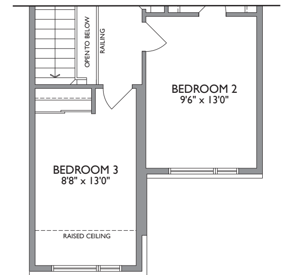
PARTIAL UPPER LEVEL ELEV. B
