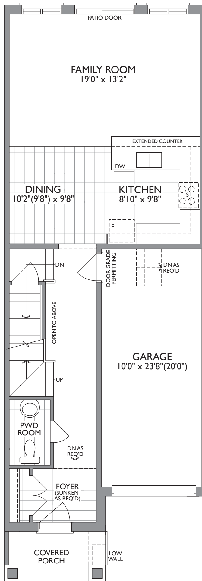
MAIN LEVEL ELEV. A & B
