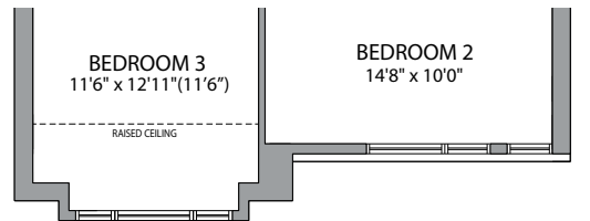
PARTIAL UPPER LEVEL ELEVATION B
