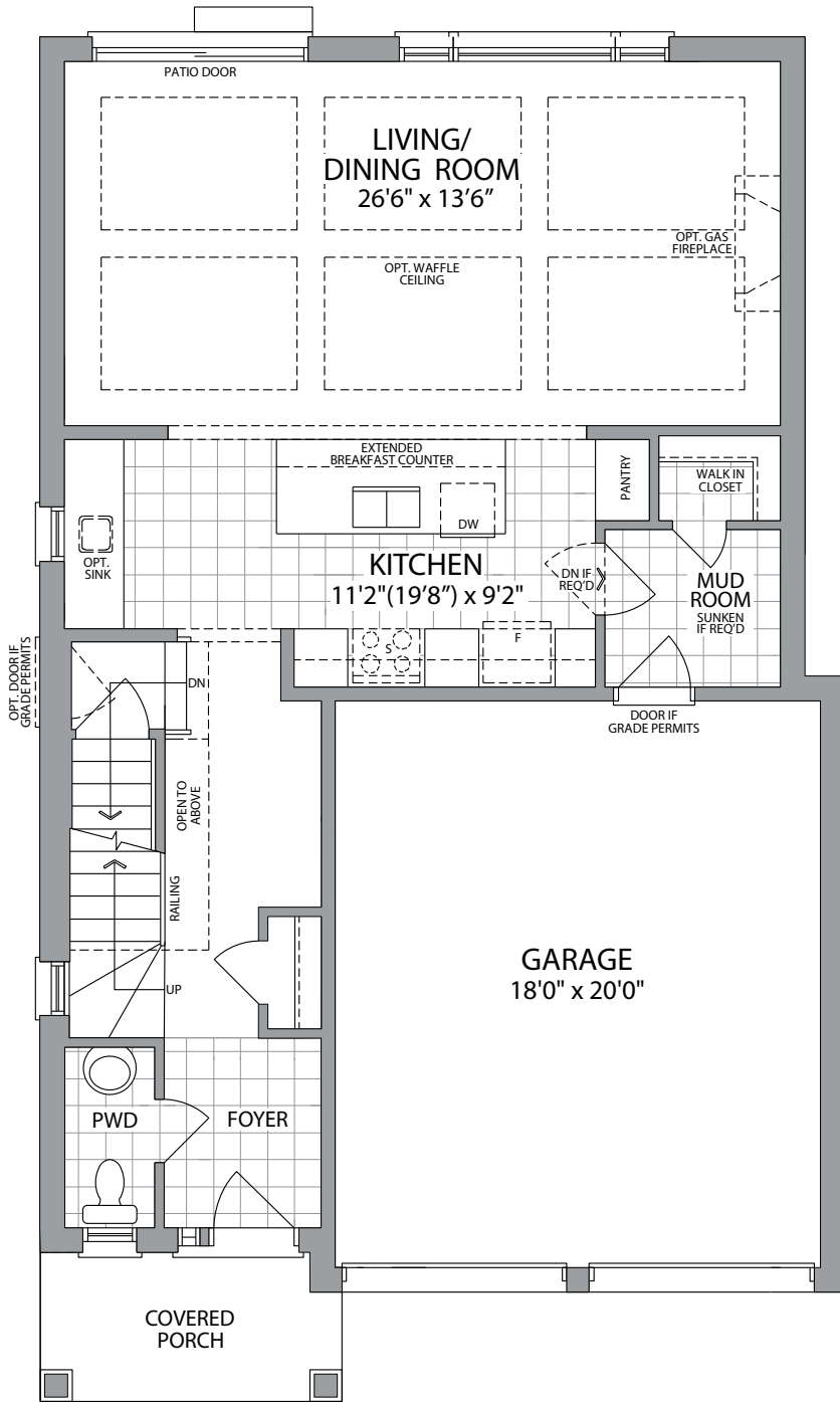
MAIN LEVEL ELEVATION C
