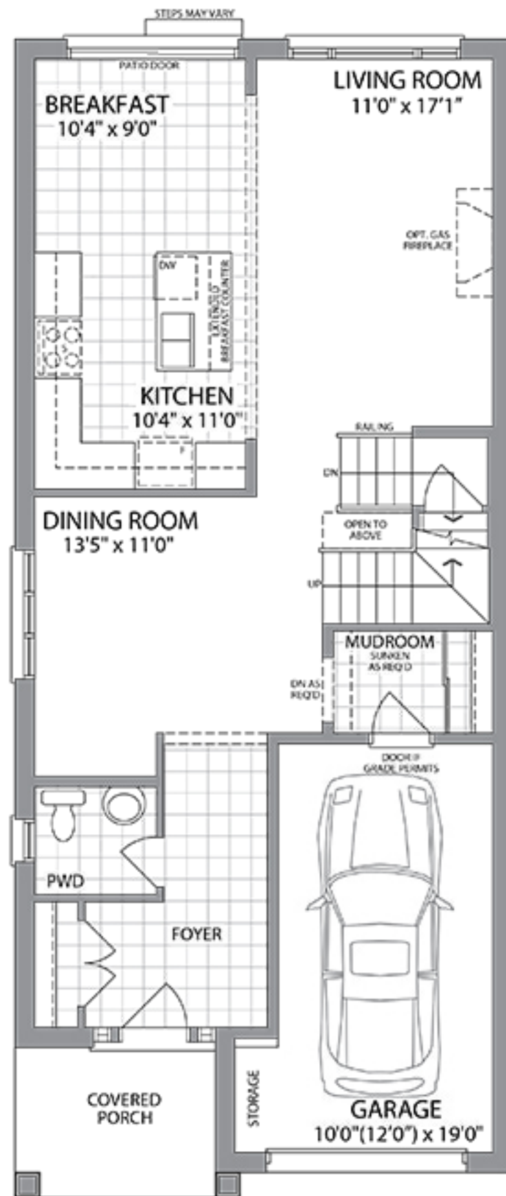
MAIN LEVEL - ELEV. A
